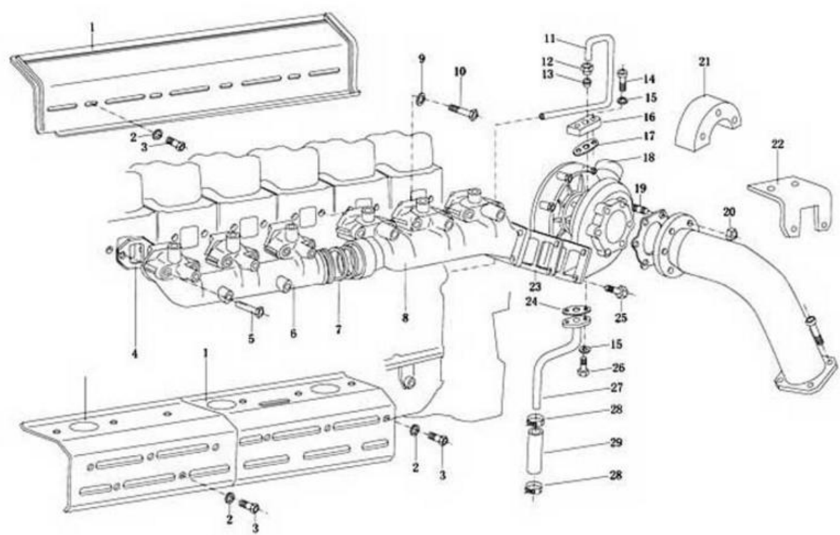
AIR INLET & EXHAUST PIPE -ONE
